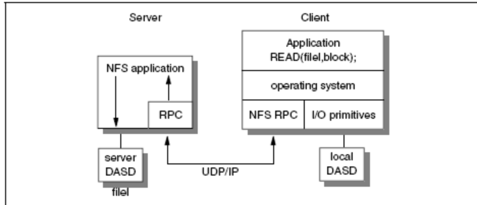
Gambar 11.95 Protokol NFS
