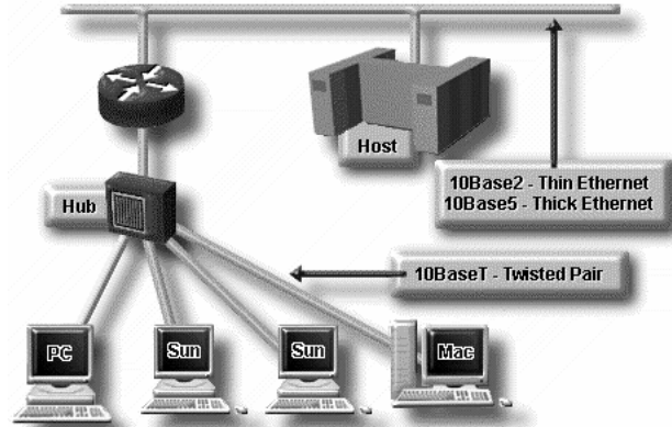
Gambar 3.31 Ethernet IEEE 802.3
