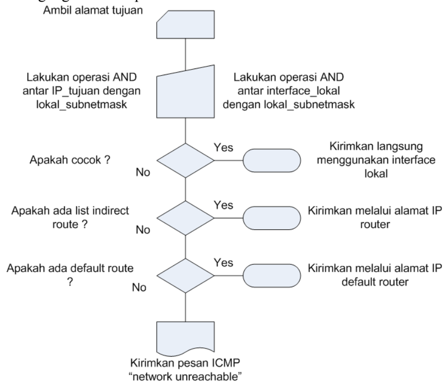
Gambar 4.64 Algoritma Routing
