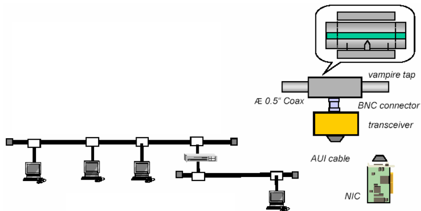
Gambar 3.32 Ethernet 10Base5
