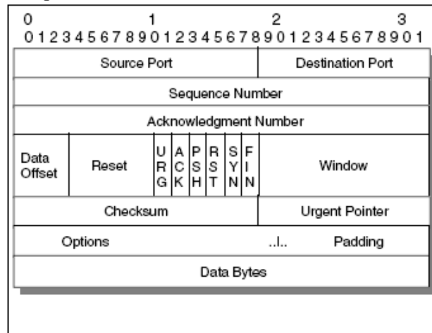
Gambar 7.78 Format TCP
