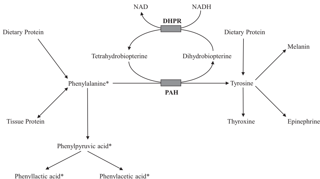
FIGURE 23.1 Metabolism of phenylalanine. PAH, phenylalanine hydroxylase; DHPR, dihydropterine reductase.
