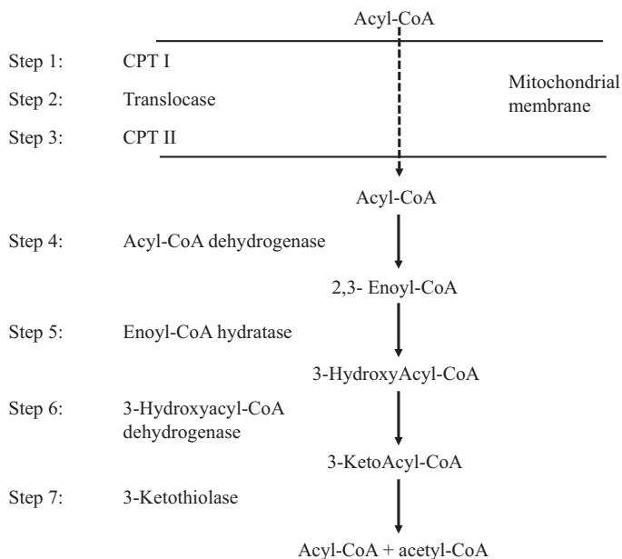
FIGURE 23.3 Simplified schematic of fatty acid \beta oxidation. CoA=coenzyme A; CPT-1, -2=carnitine-palmitoyl transferase-1, -2.
