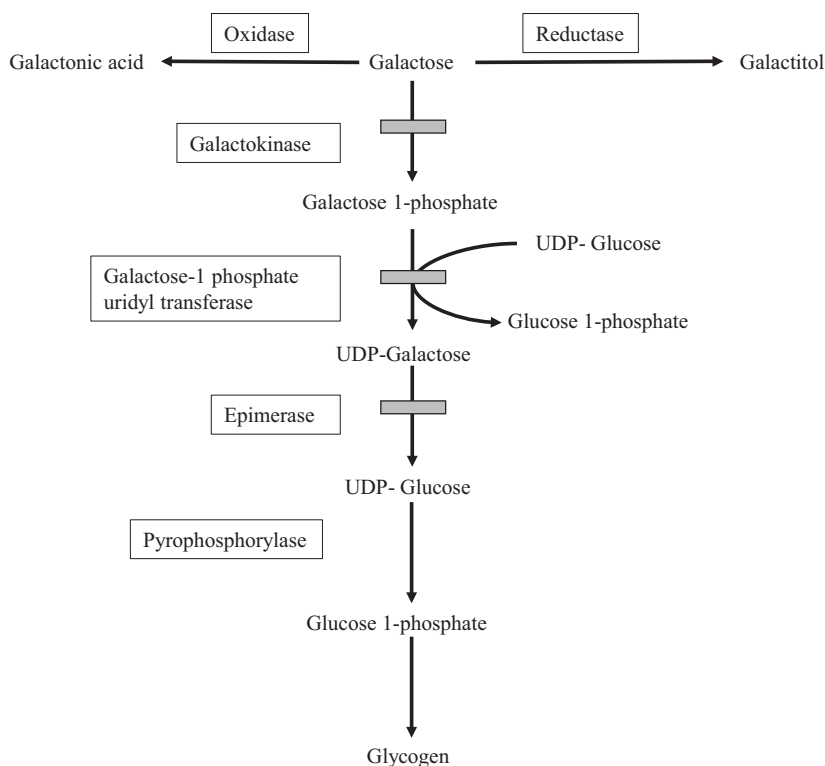
FIGURE 23.2 Galactose metabolism and enzyme blocks (indicated by gray bars) that lead to galactosemia.
