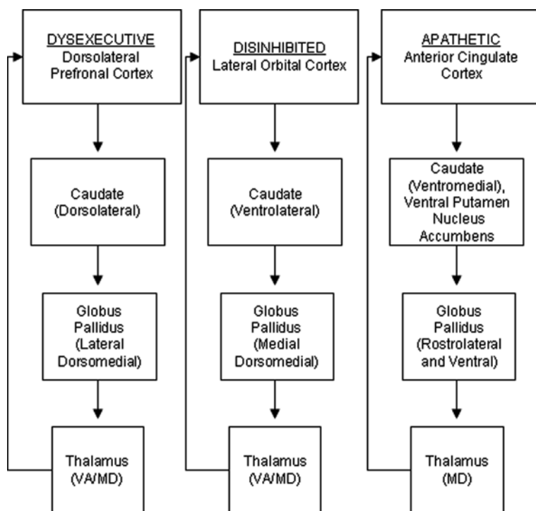
Fig. 1. Frontal–subcortical circuits.
