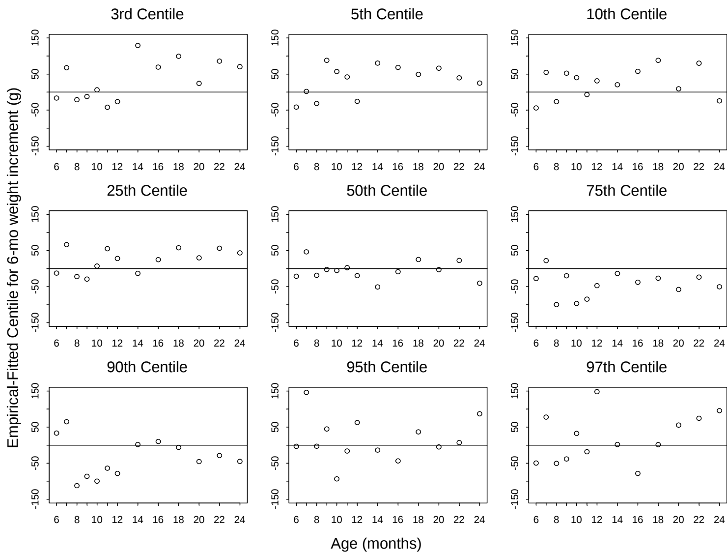
Figure A3.46 Centile residuals from fitting selected model for 6-month weight velocity for girls
