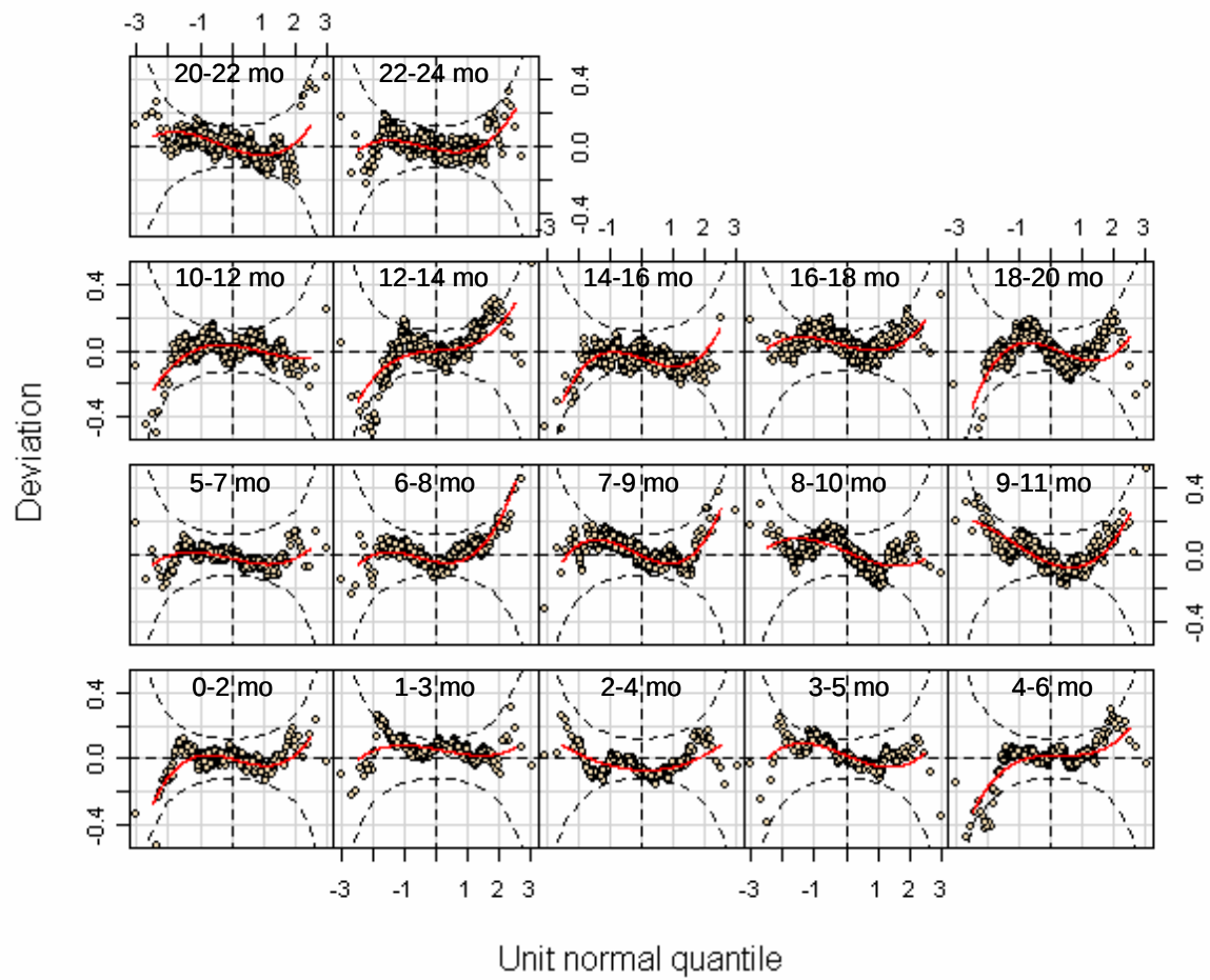
Figure A3.11 Worm plots from selected model [BCPE( x = \text{age}^{0.05} , df(\mu) = 12 , df(\sigma) = 6 , df(v) = 3 , \tau = 2 )] for 2-month weight velocity for boys
