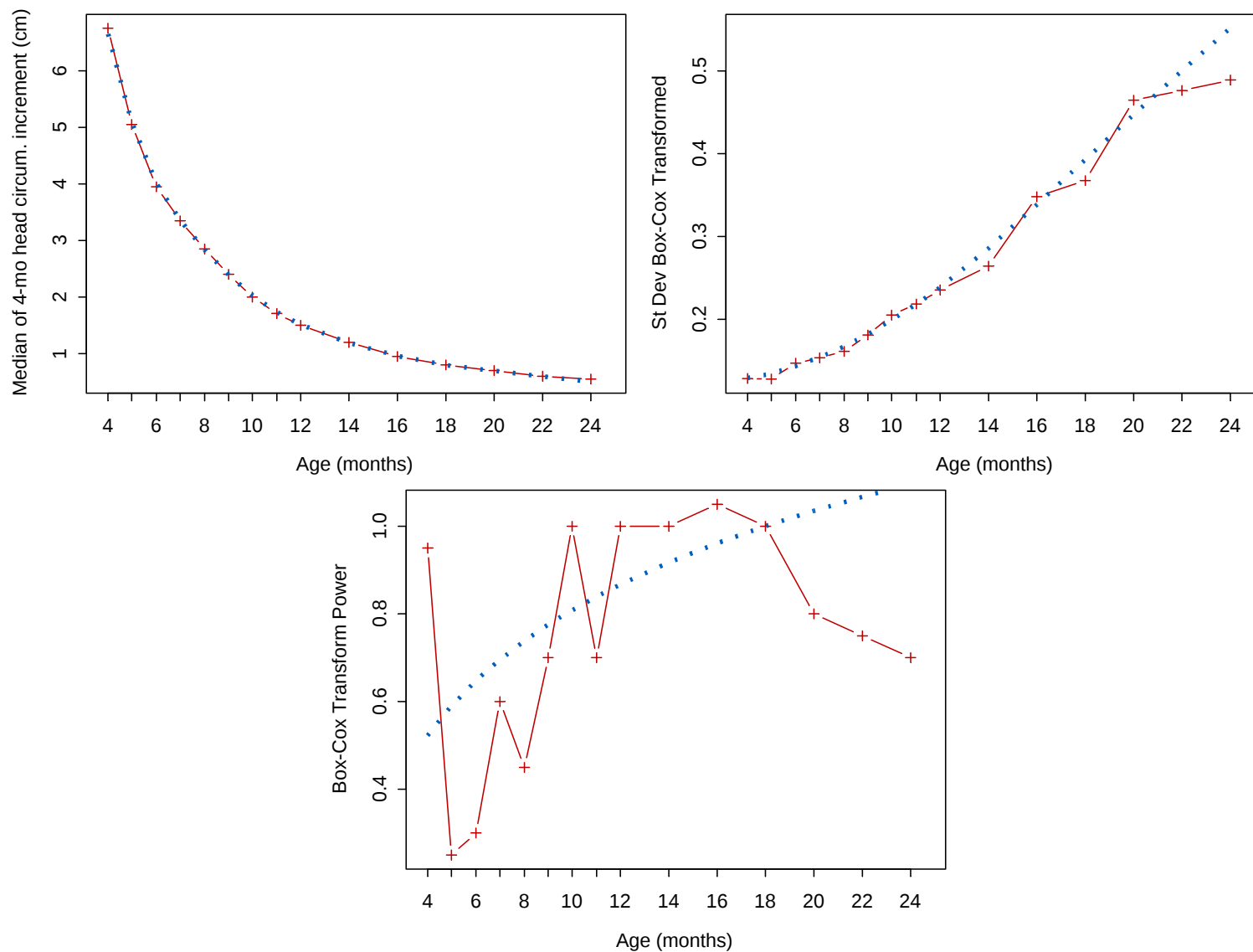
Figure A5.27 Fitting of the \mu , \sigma , and v curves of selected model for 4-month head circumference velocity for girls
