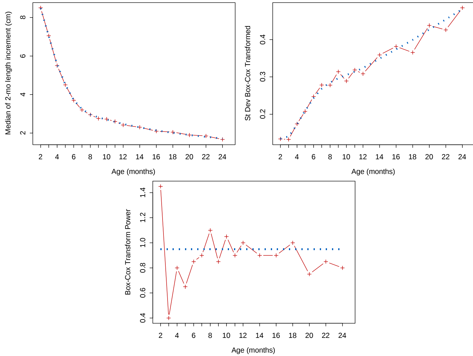
Figure A4.2 Fitting of the \mu , \sigma , and \nu curves of selected model for 2-month length velocity for boys
