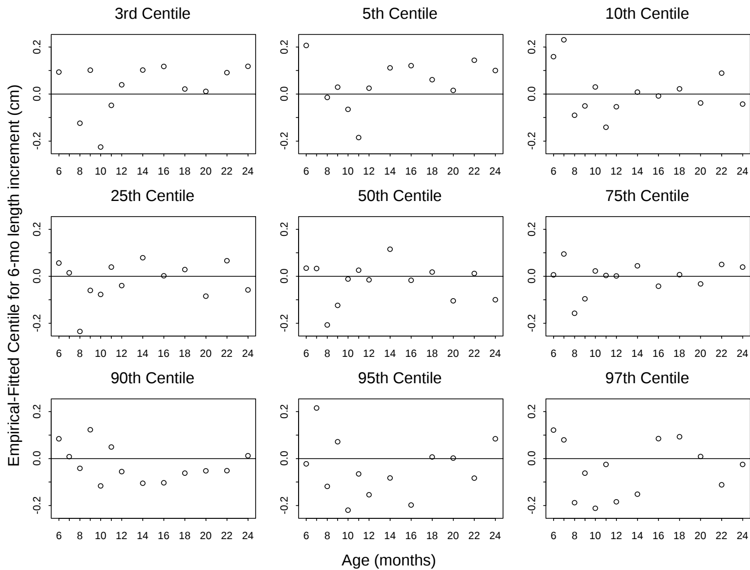
Figure A4.31 Centile residuals from fitting selected model for 6-month length velocity for boys
