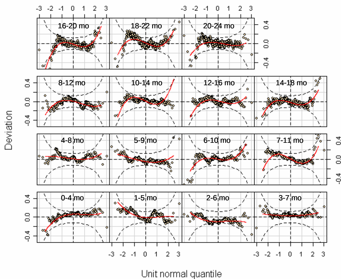
Figure A5.21 Worm plots from selected model [BCPE( x = \text{age}^{0.05} , df(\mu) = 10 , df(\sigma) = 5 , df(v) = 3 , \tau = 2 )] for 4-month head circumference velocity for boys
