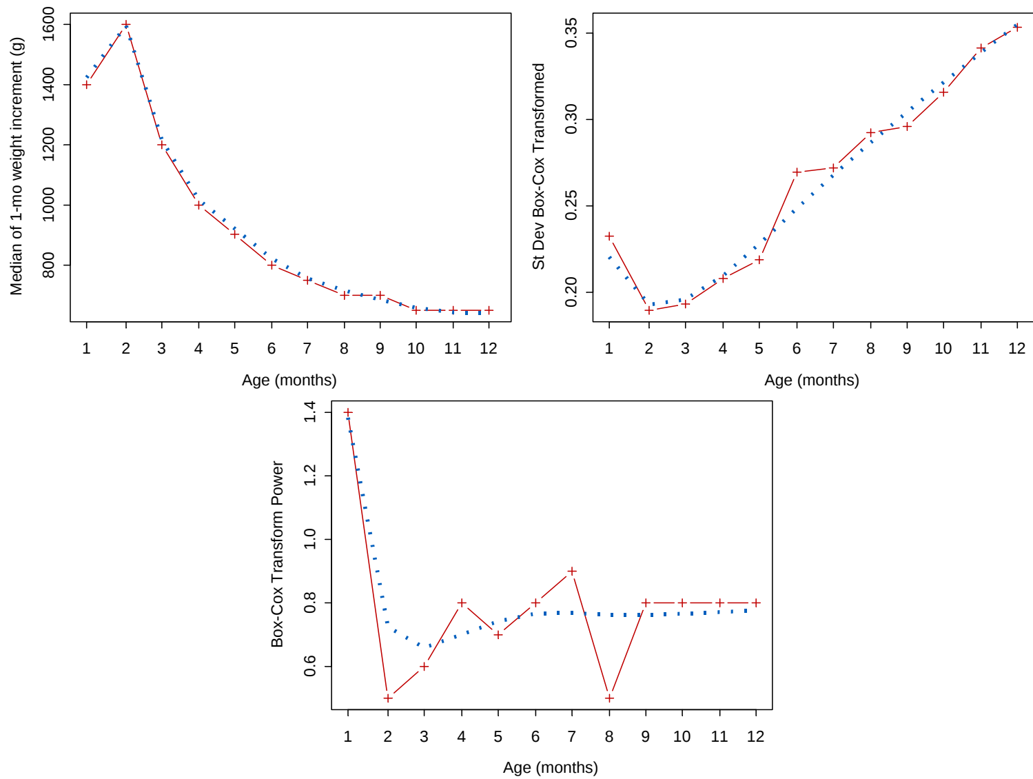
Figure A3.2 Fitting of the \mu , \sigma , and v curves of selected model for 1-month weight velocity for boys
