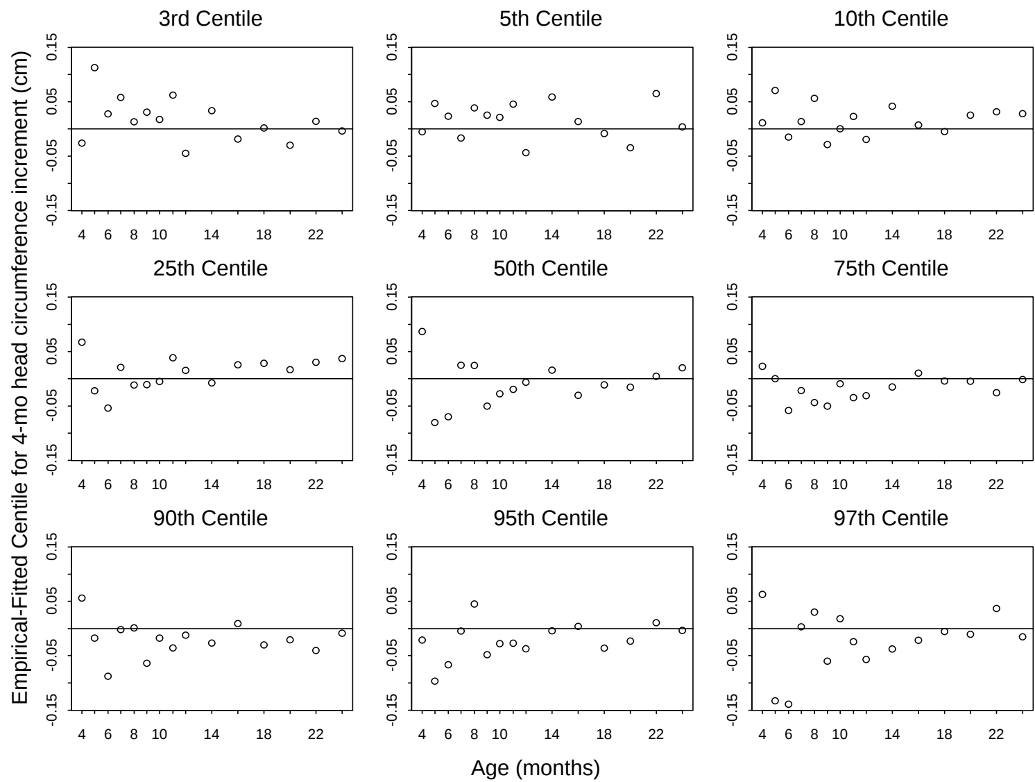
Figure A5.25 Centile residuals from fitting selected model for 4-month head circumference velocity for boys
