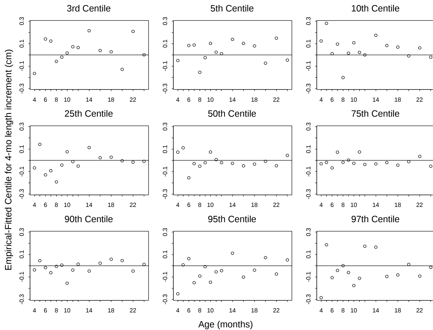
Figure A4.21 Centile residuals from fitting selected model for 4-month length velocity for boys
