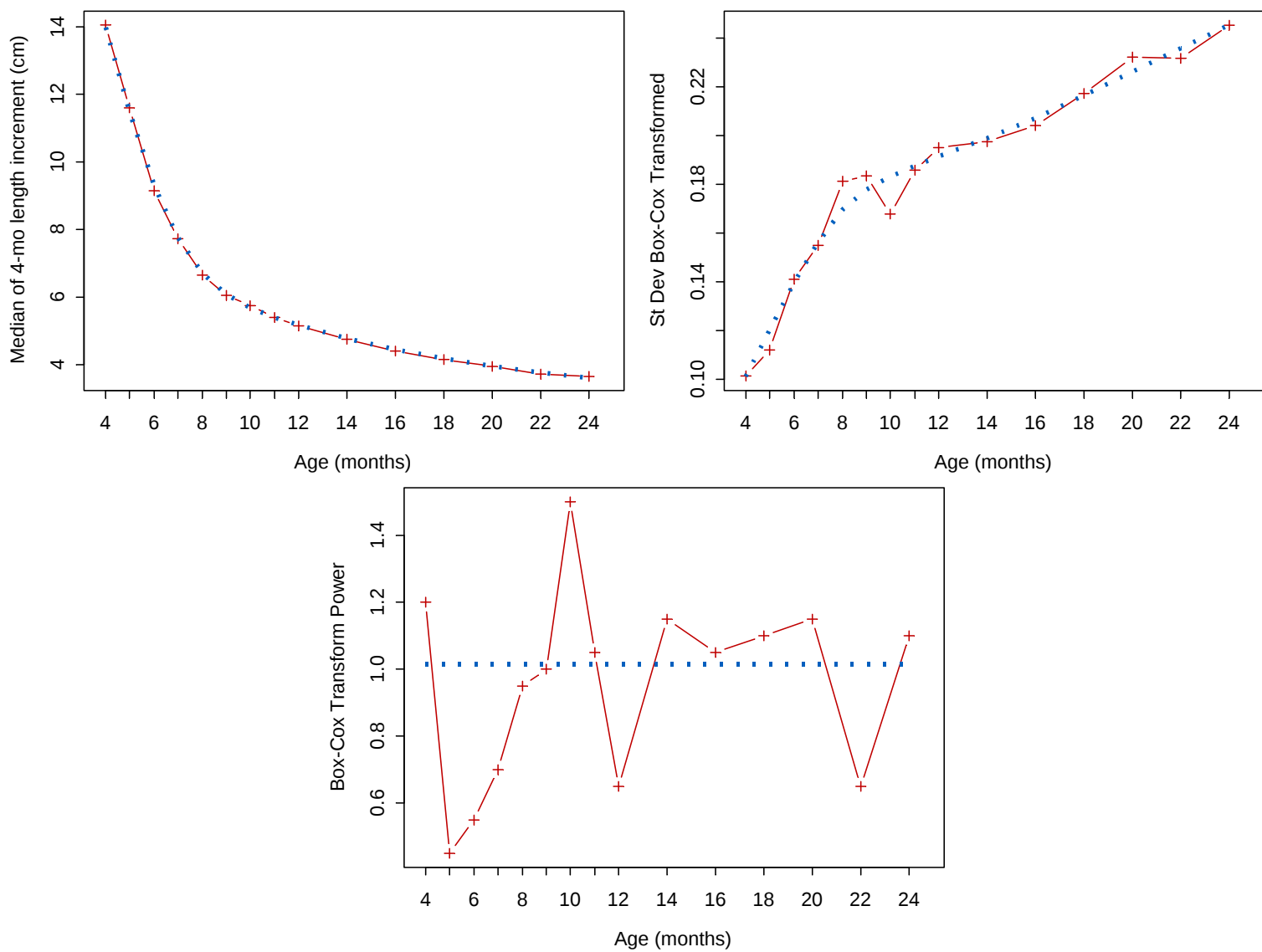
Figure A4.18 Fitting of the \mu , \sigma , and v curves of selected model for 4-month length velocity for boys
