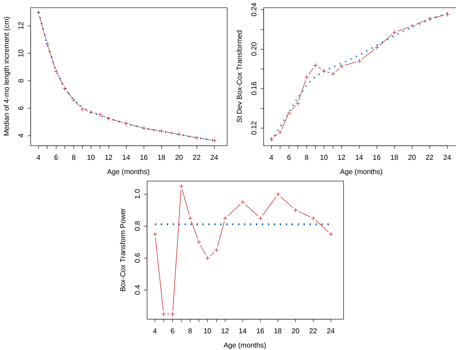
Figure A4.23 Fitting of the \mu , \sigma , and \nu curves of selected model for 4-month length velocity for girls
