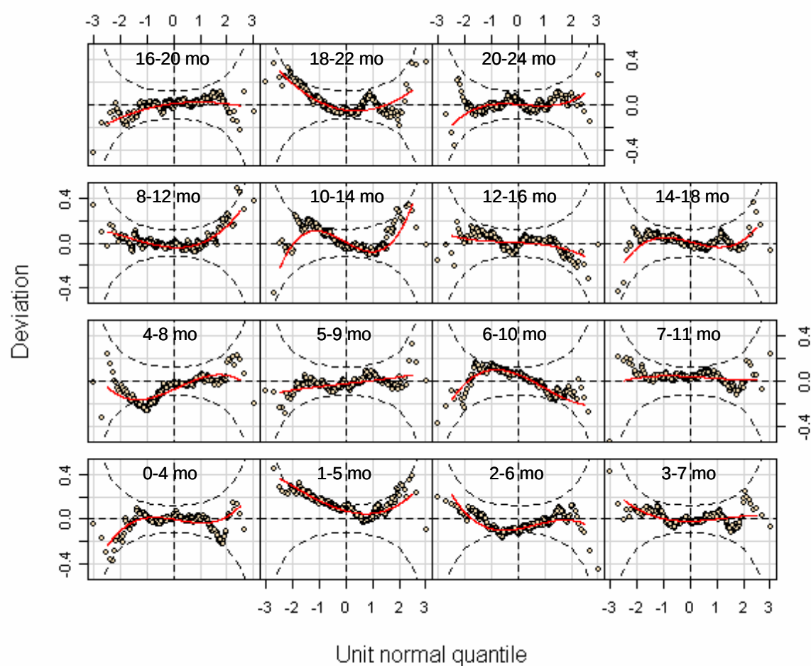
Figure A4.17 Worm plots from selected model [BCPE( x = \text{age}^{0.05} , \text{df}(\mu) = 8 , \text{df}(\sigma) = 5 , \text{df}(\nu) = 1 , \tau = 2 )] for 4-month length velocity for boys
