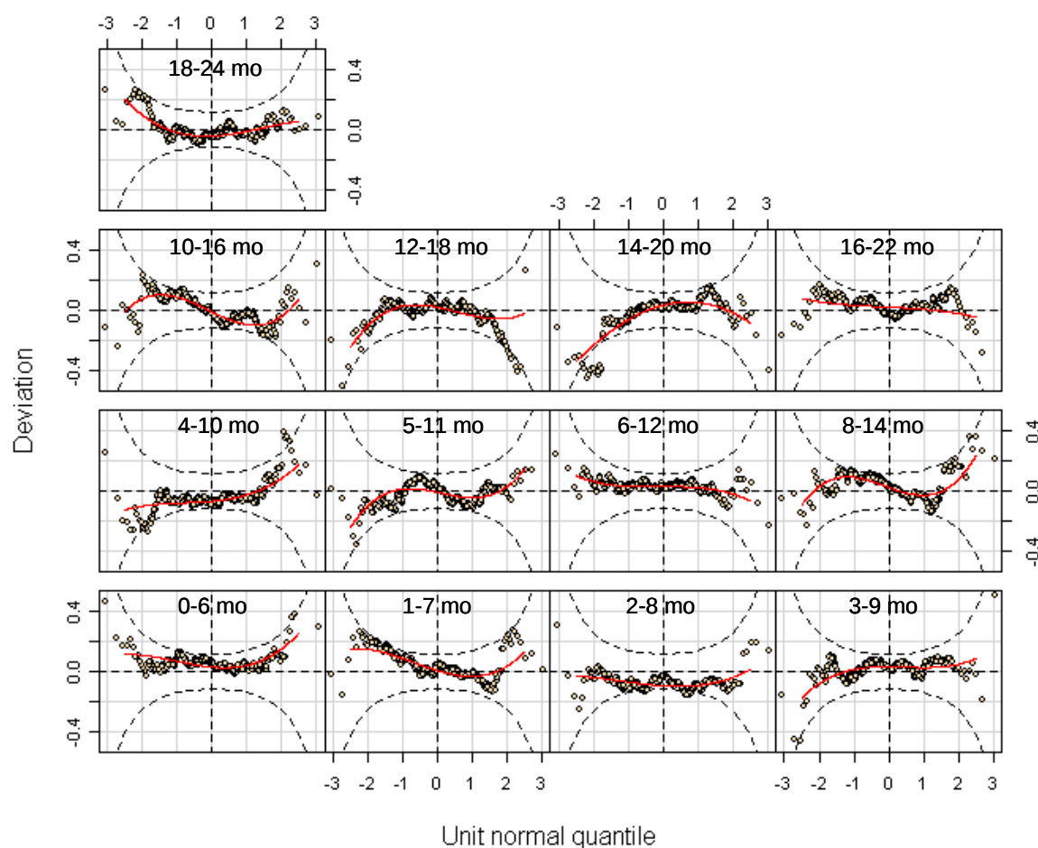
Figure A4.32 Worm plots from selected model [BCPE(x=age^{0.05}, df(\mu)=7, df(\sigma)=4, df(v)=1, \tau=2)] for 6-month length velocity for girls
