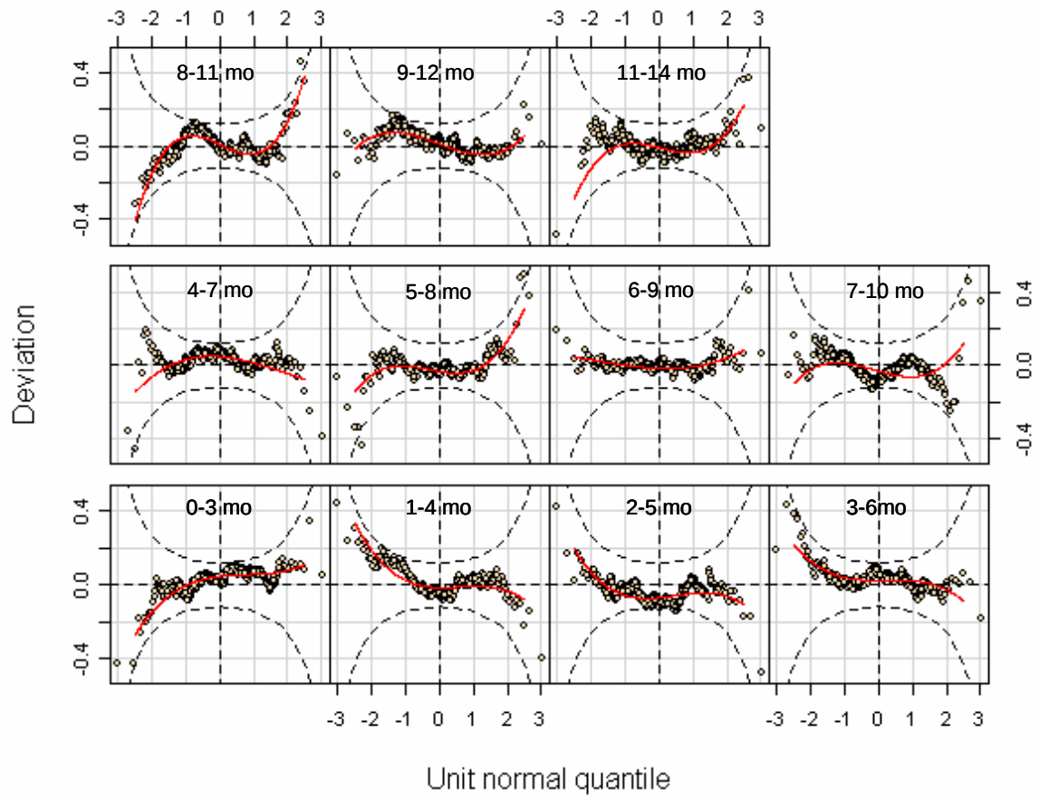
Figure A5.11 Worm plots from selected model [BCPE( x = \text{age}^{0.05} , df(\mu)=7 , df(\sigma)=4 , df(v)=4 , \tau=2 )] for 3-month head circumference velocity for boys
