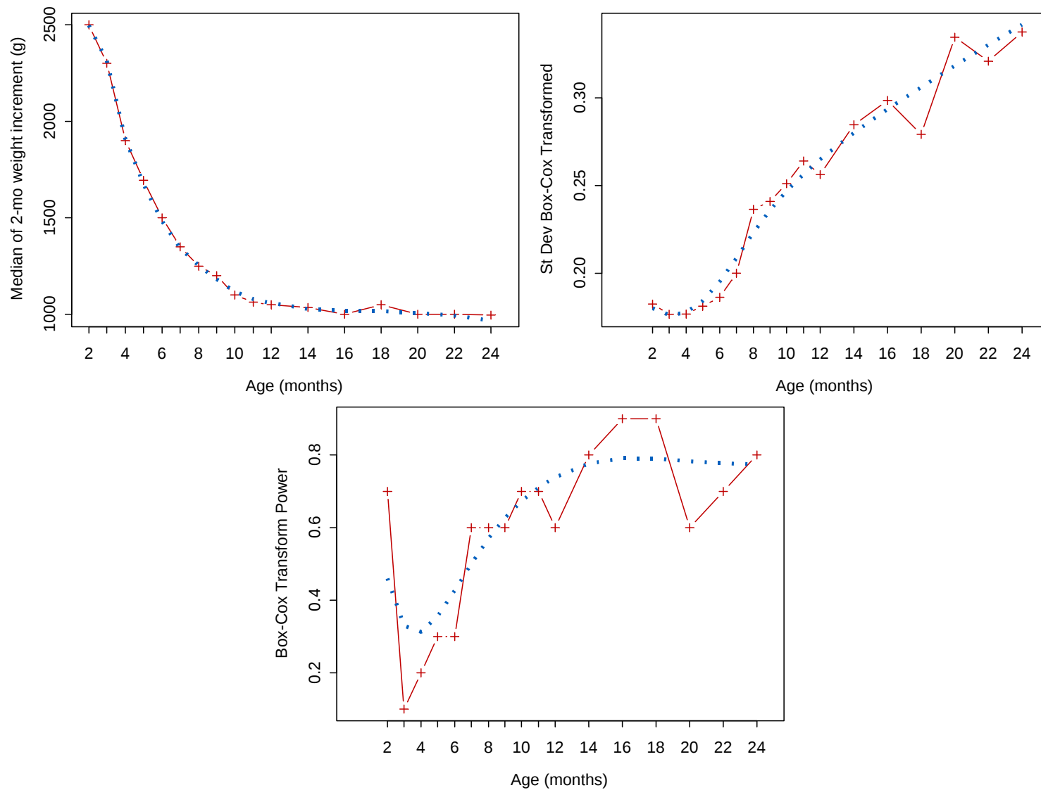
Figure A3.17 Fitting of the \mu , \sigma , and v curves of selected model for 2-month weight velocity for girls
