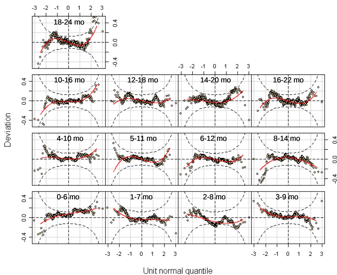
Figure A5.31 Worm plots from selected model [BCPE( x = \text{age}^{0.05} , df(\mu) = 9 , df(\sigma) = 4 , df(v) = 2 , \tau = 2 )] for 6-month head circumference velocity for boys
