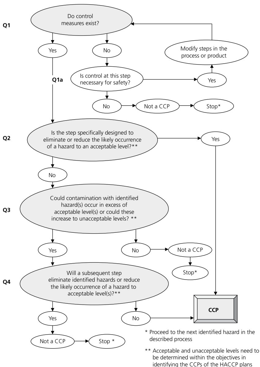
Figure 3.2 Example of decision tree for process steps. Source: Adapted from Codex (2009b).
