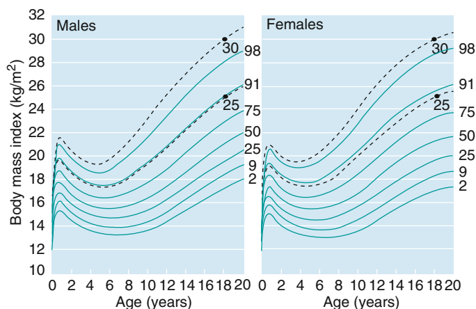
FIGURE 5.1 Gentiles for body mass index for British males and females. Gentile curves are spaced two thirds of z score apart. Also shown are body mass index values of 25 and 30 \text{kg/m}^2 at age 18, with extra centile curves drawn through them
