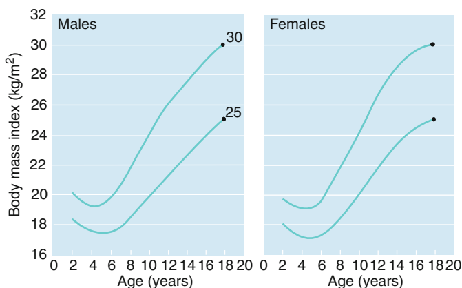
FIGURE 5.2 International cut off points for body mass index by sex for overweight and obesity, passing through body mass index 25 and 30 kg/m 2 at age 18 (data from Brazil, Britain, Hong Kong, Netherlands, Singapore, and United States)
