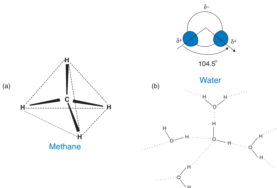
Figure 1.3 (a) Three-dimensional structure of the methane molecule and (b) the molecular structure of water. (a) The hydrogen atoms of methane (CH 4 ) are arranged symmetrically in space, at the corners of a tetrahedron. (b) The molecular structure of water. Top: view of the 'electron cloud' surrounding the molecule; bottom, interactions between water molecules. The molecule has a degree of polarity , and this leads to electrical interactions between neighboring molecules by the formation of hydrogen bonds . These bonds are not strong compared with covalent bonds, and are constantly being formed and broken. Nevertheless, they provide sufficient attraction between the molecules to account for the fact that water is a liquid at room temperature whereas the non-polar methane is a gas.
