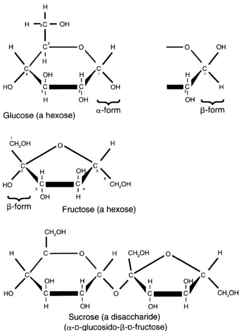
Figure 1.7 Some simple sugars and disaccharides. Glucose and fructose are shown in their 'ring' form. Even this representation ignores the true three-dimensional structure, which is 'chair' shaped: if the middle part of the glucose ring is imagined flat, the left-hand end slopes down and the right-hand end up. Glucose forms a six-membered ring and is described as a pyranose; fructose forms a five-membered ring and is described as a furanose. In solution the \alpha - and \beta -forms are in equilibrium with each other and with a smaller amount of the straight-chain form. The orientation of the oxygen on carbon atom 1 becomes fixed when glucose forms links via this carbon to another sugar, as in sucrose; \alpha - and \beta -links then have quite different properties (e.g., cellulose vs starch or glycogen).
